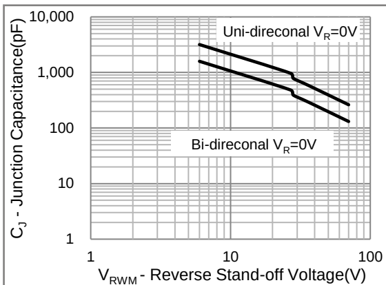
Fig.4 Typical Capacitance
