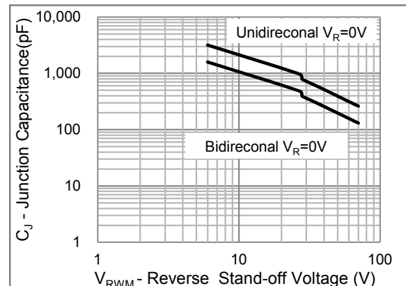
Fig.4 Typical Capacitance
