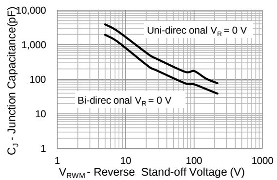
Fig.4 Typical Capacitance
