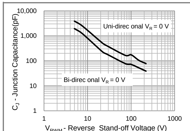
Fig.4 Typical Capacitance
