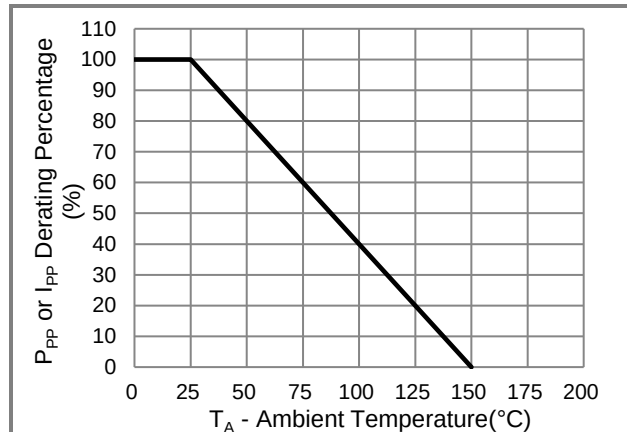
Fig.2 Derating Curve
