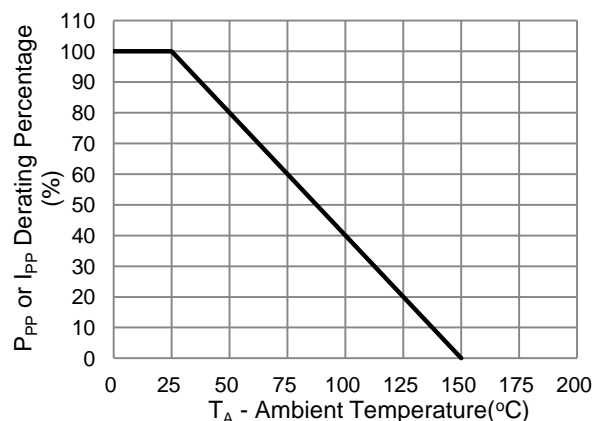
Fig.2 Derating Curve
