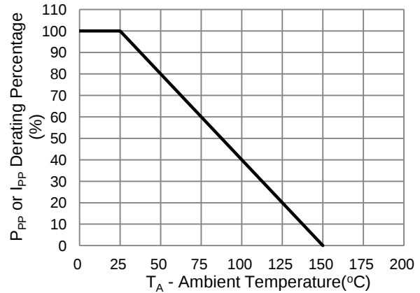
Fig.2 Derating Curve
