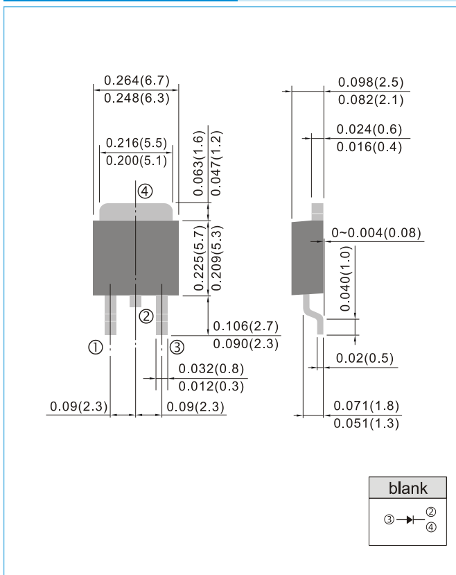
TO-252
