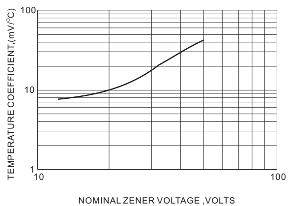
Fig.2 TEMPERATURE COEFFICIENTS
