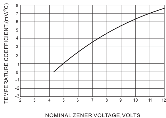
Fig.1 TEMPERATURE COEFFICIENTS
