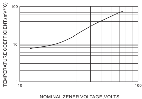
Fig.2 TEMPERATURE COEFFICIENTS
