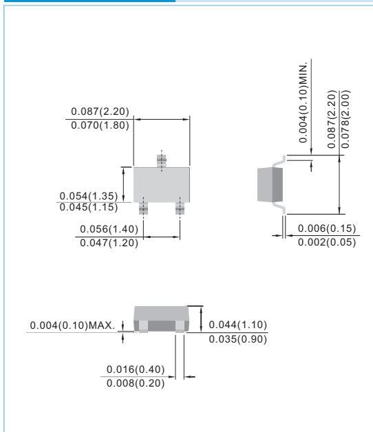
SOT-323 Unit: inch (mm)
