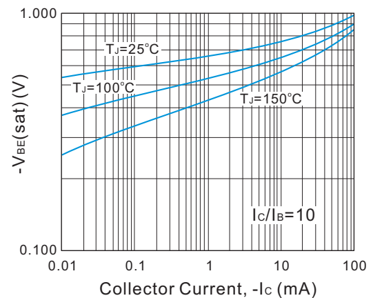
Fig. 4. Typical V_{BE(sat)} vs Collector Current
