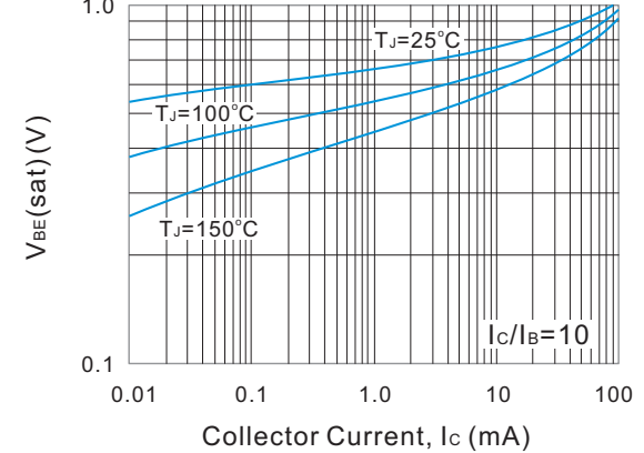
Fig. 4. Typical V_{BE(sat)} vs Collector Current
