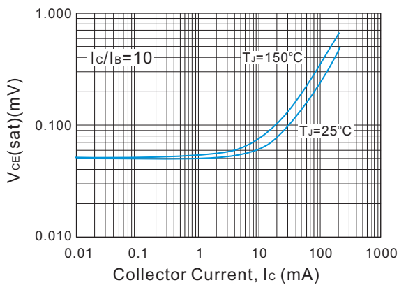
Fig. 3. Typical V_{CE(sat)} vs. Collector Current
