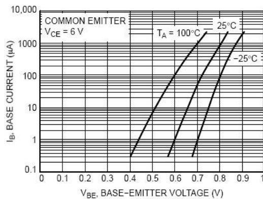
Fig. 5. Base-Emitter Voltage
