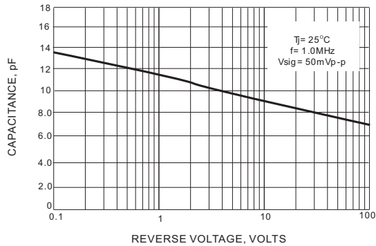
FIG.1 TYPICAL JUNCTION CAPACITANCE
