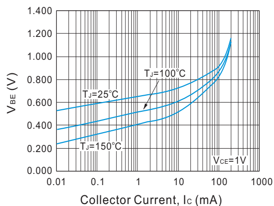
Fig. 2. Typical V_{BE} vs. Collector Current
