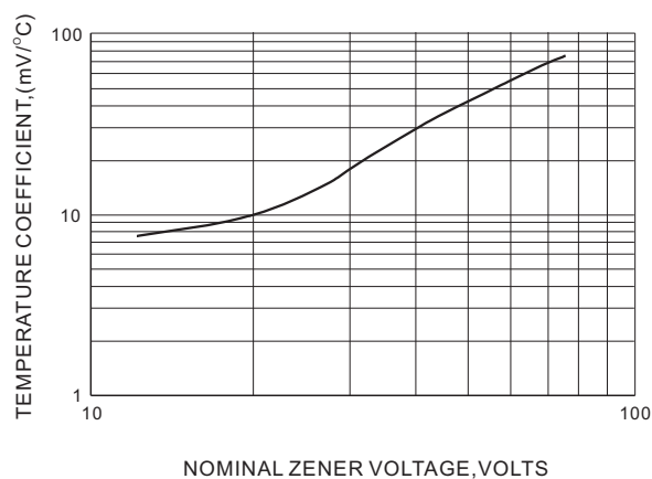
Fig.2 TEMPERATURE COEFFICIENTS
