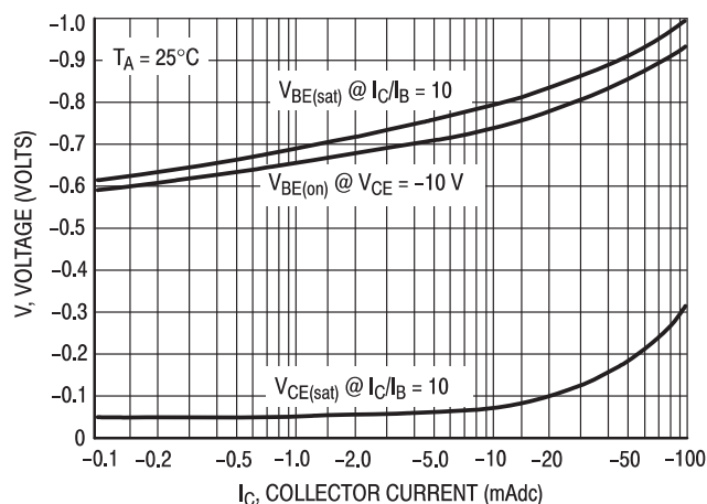
Figure 8 . "Saturation" and "On" Voltages
