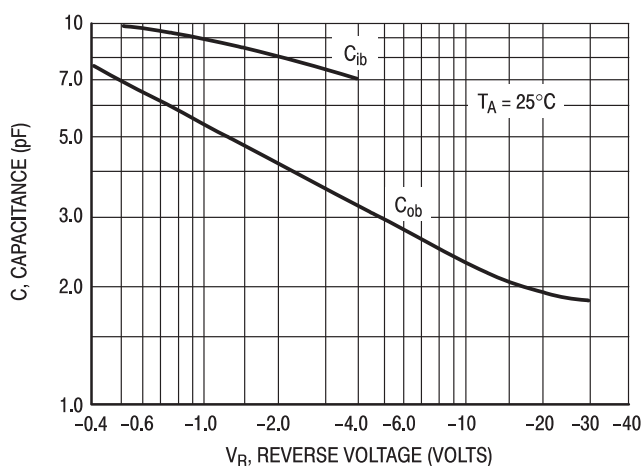
Figure 11 . Capacitances
