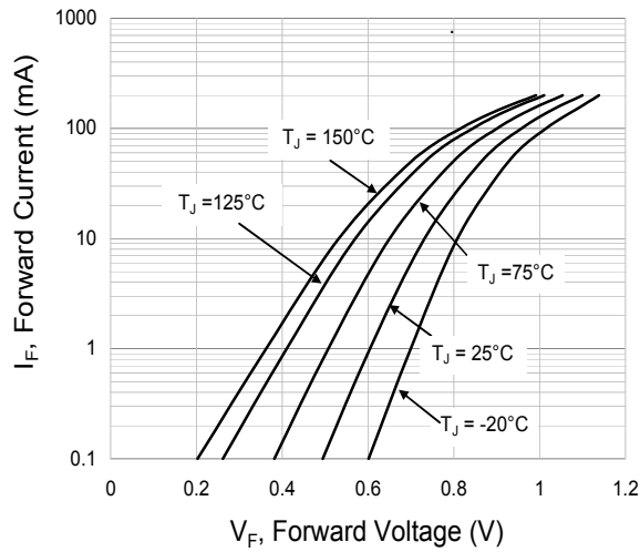
FIG. 1-TYPICAL FORWARD CHARACTERISTIC
