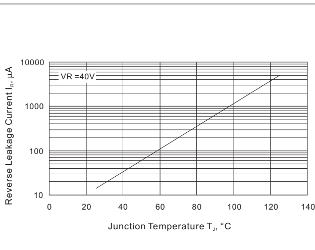
FIG. 1 Reverse Leakage Current vs. Junction Temperature
