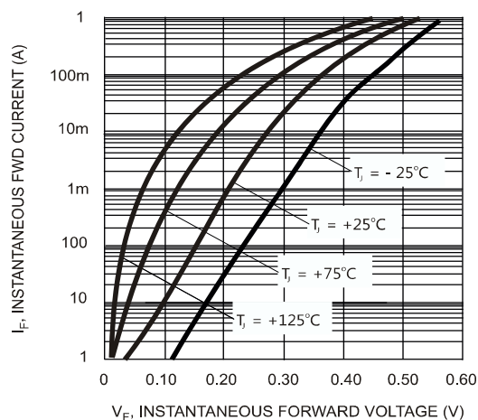
FIG.2 TYPICAL FWD CHARACTERISTICS
