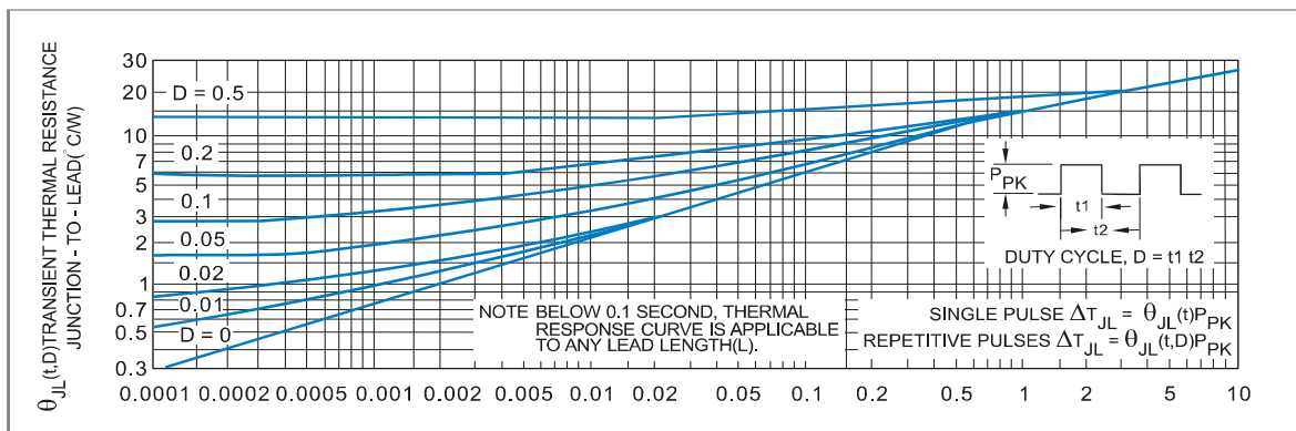
FIGURE 3. TYPICAL THERMAL RESPONSE,
