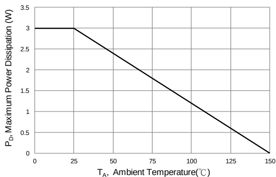
Fig.1 Steady-State Power Derating Curve
