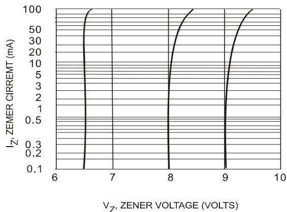
FIGURE 6. V_Z=6.8 THRU 10 VOLTS
