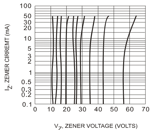
FIGURE 7. V_Z=12 THRU 51 VOLTS
