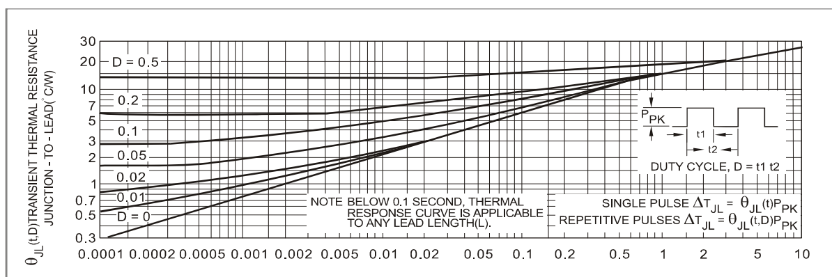
FIGURE 3. TYPICAL THERMAL RESPONSE,
