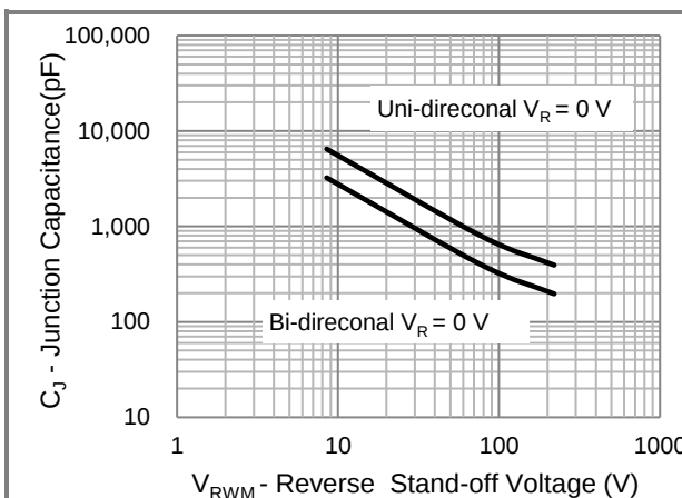
Fig.4 Typical Capacitance
