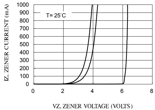
Fig.7-ZENER VOLTAGE VERSUS ZENER CURRENT VZ=3.6 THRU 6 VOLTS
