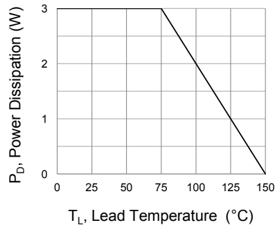
Fig.1 Steady-State Power Derating Curve
