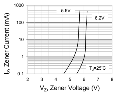
Fig.4 Typical Zener Characteristics
