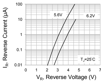
Fig.3 Typical Leakage Characteristics
