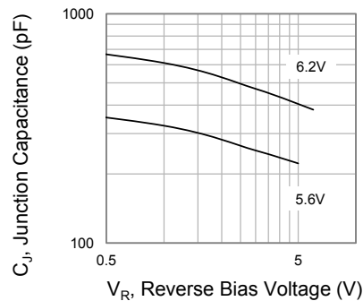
Fig.2 Typical Junction Capacitance
