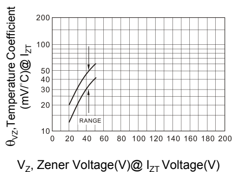
Fig.7 Units 10 To 51 Volts
