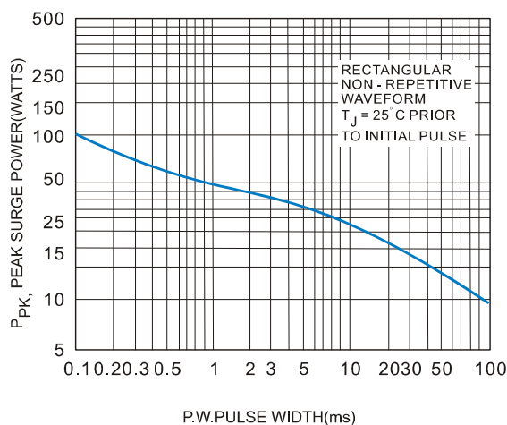
FIGURE 2. MAXIMUM SURGE POWER
