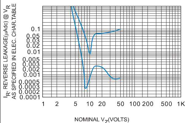
FIGURE 3. TYPICAL REVERSE LEAKAGE
