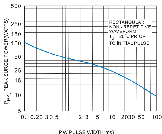
FIGURE 2. MAXIMUM SURGE POWER
