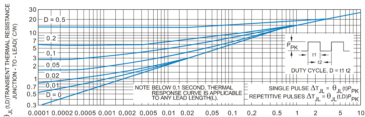
FIGURE 1. TYPICAL THERMAL RESPONSE L,
