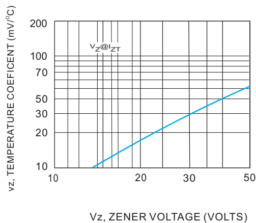
Fig.3 Temperature coefficient v.s. zener voltage, Vz(V)
