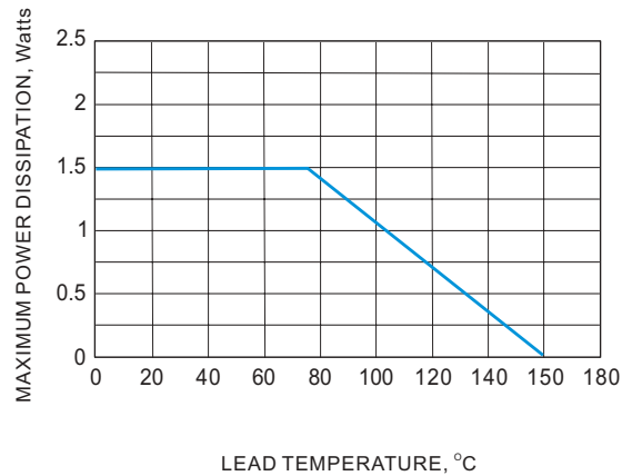
Fig.1 Steady State Power Derating
