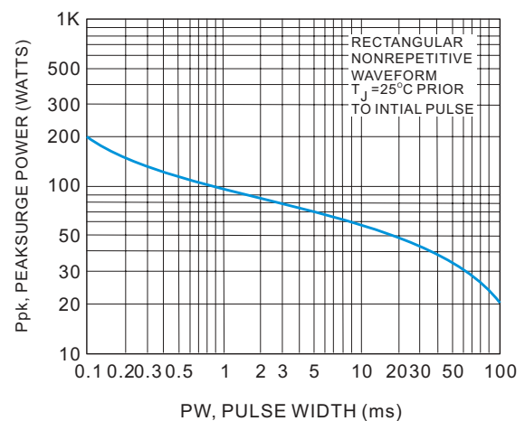
Fig.6 Maximum Surge Power
