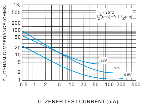
Fig.4 Zener impedance v.s. zener current
