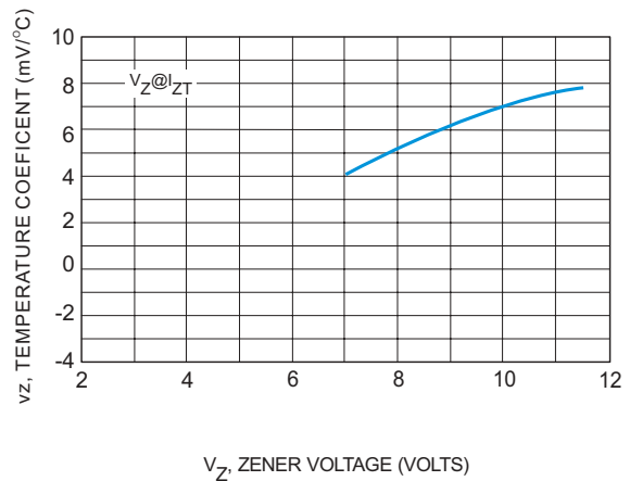
Fig.2 Temperature coefficient v.s. zener voltage, Vz(V)
