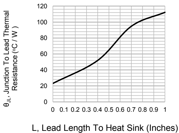
Fig.7 Thermal Resistance Versus Lead Length
