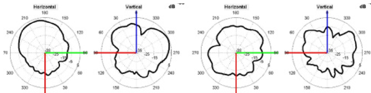
2450 and 5500 MHz Radiation Pattern
