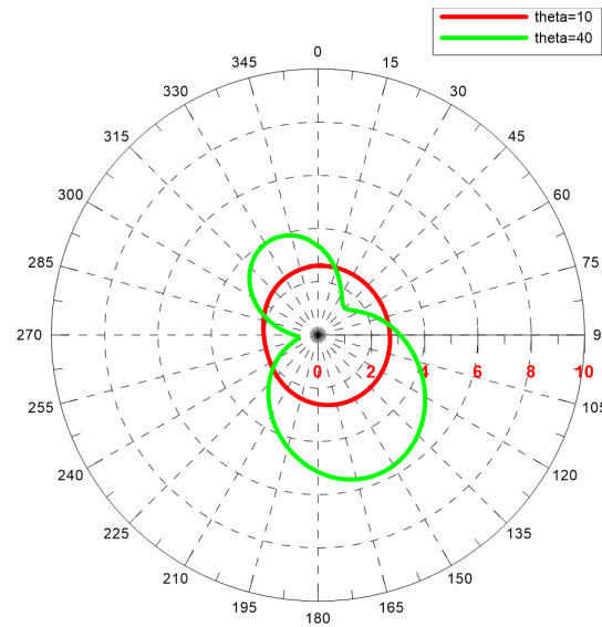
Axial Ratio [dB] - Azimuth Cuts
