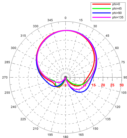
RHCP Realized Gain [dBic] - Elevation Cuts
