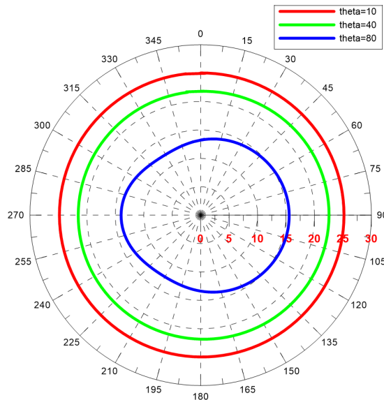
RHCP Realized Gain [dBic] - Azimuth Cuts
