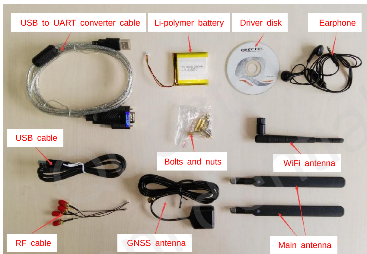
Figure 3: EVB Accessories
