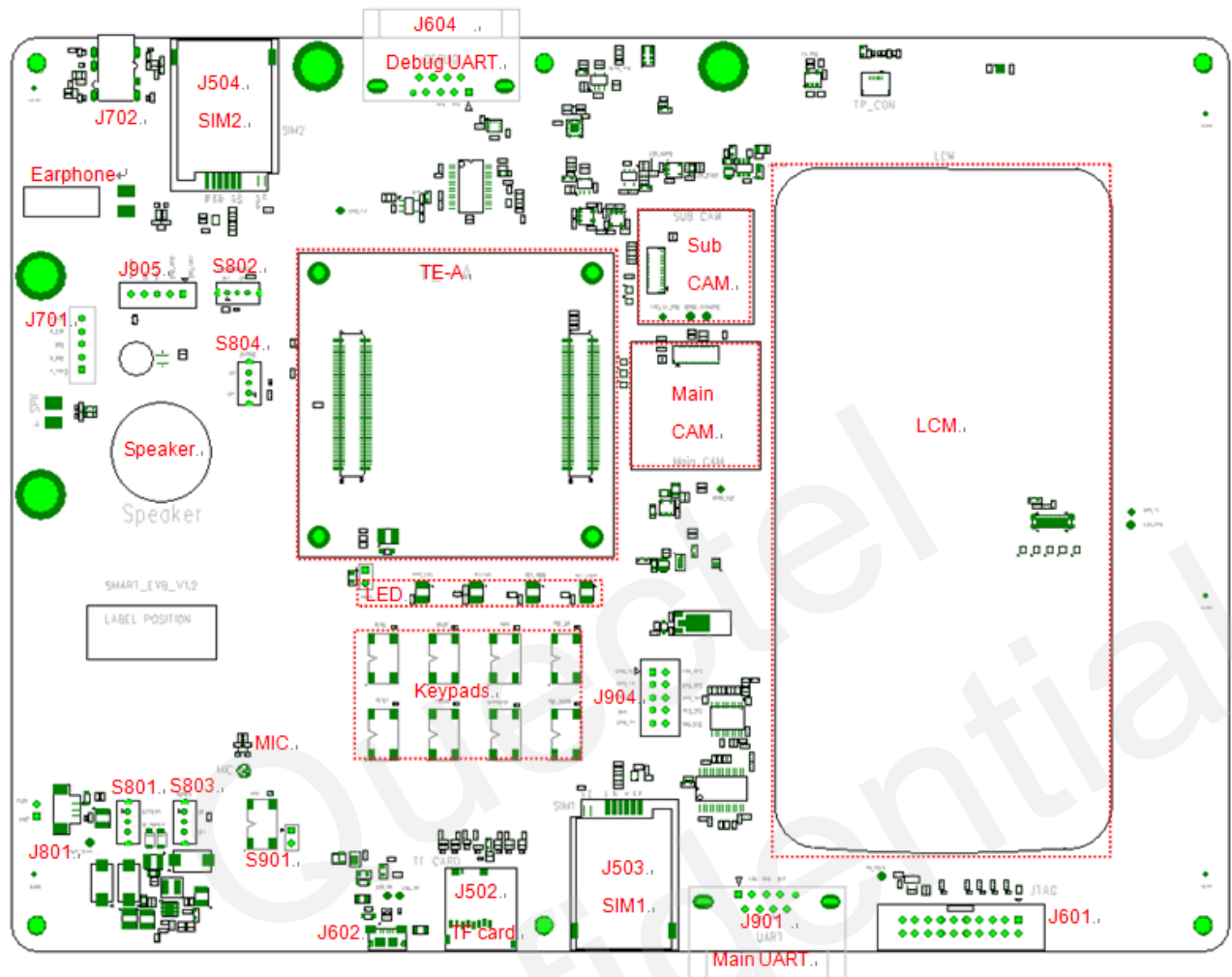
Figure 1: Interface Overview
