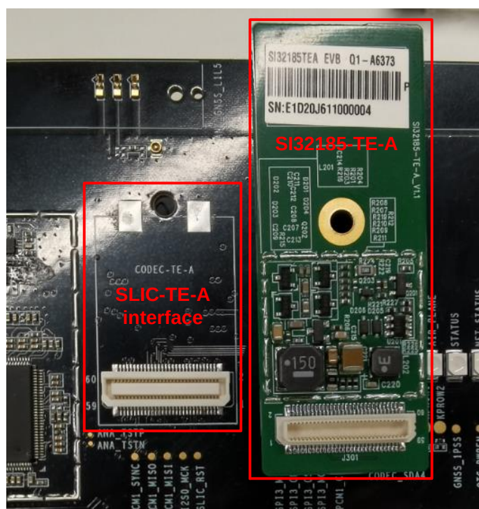
Figure 8: Connection Between SI32185-TE-A and EVB
