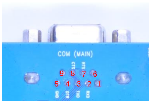
Figure 33: Pin Assignment of J0502
