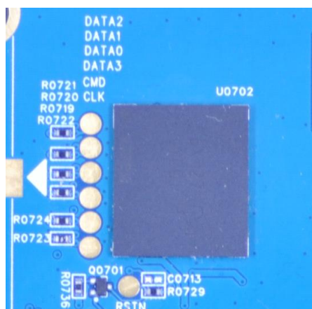
Figure 28: eMMC Device
