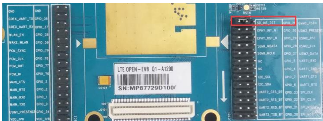
Figure 30: eMMC Function GPIO Configuration
