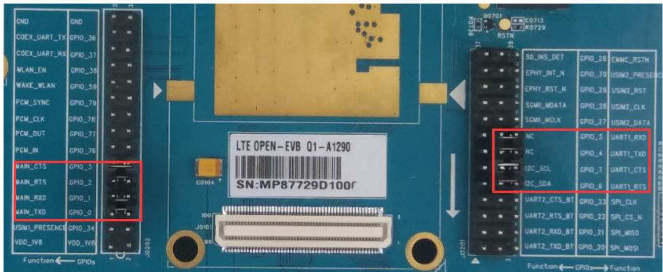
Figure 35: COM (MAIN) & COM (UART1) Function GPIO Configuration
