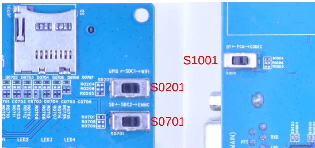
Figure 40: S0201/S0701/S1001 Switch
