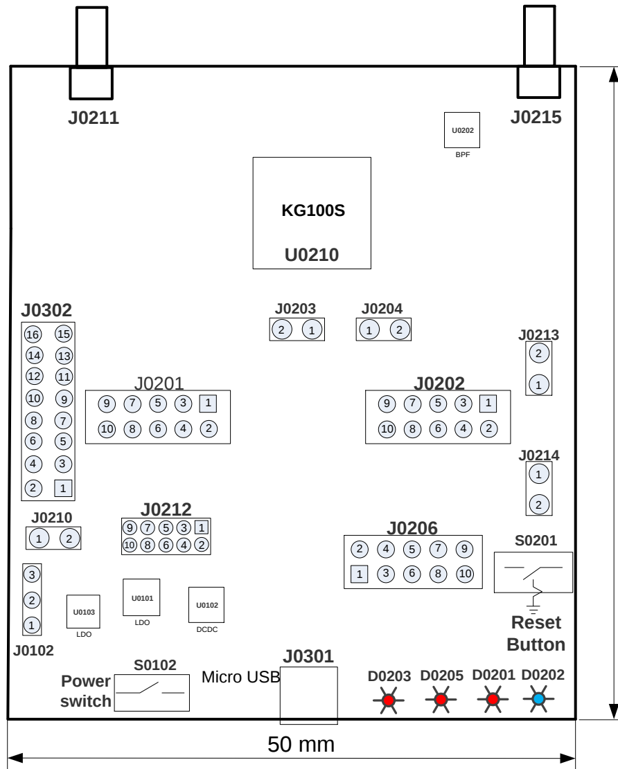
Figure 3: Component Placement of KG100S TE-B
