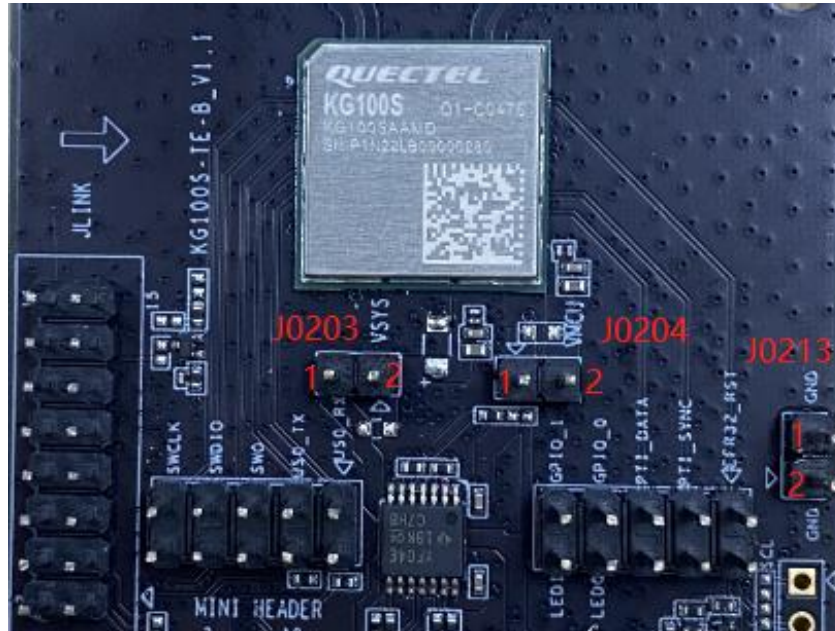
Figure 14: Test PointsTable
