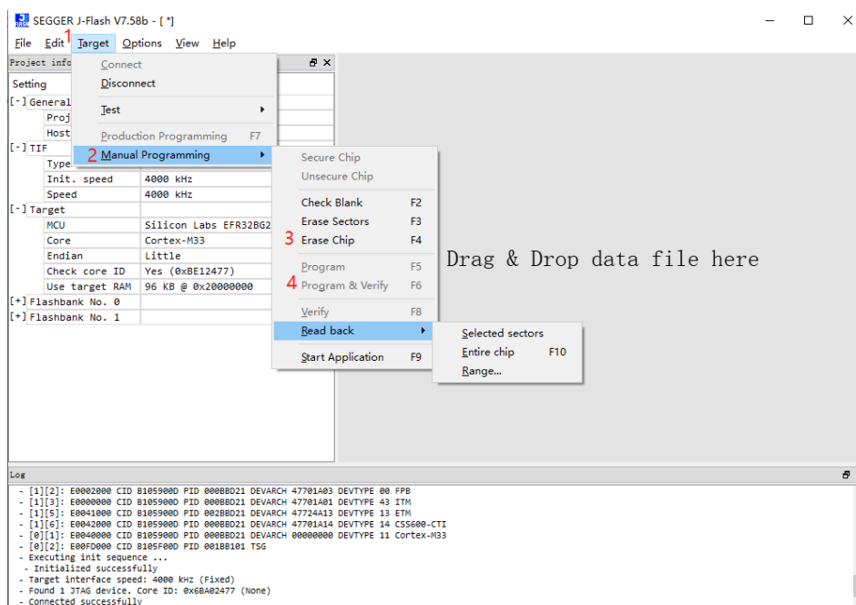
Figure 22: Firmware Upgrade (3)
