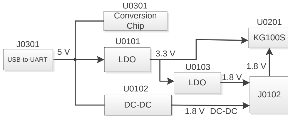
Figure 6: Power Supply for KG100S TE-B
