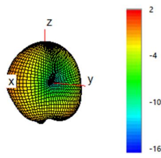
960 MHz
