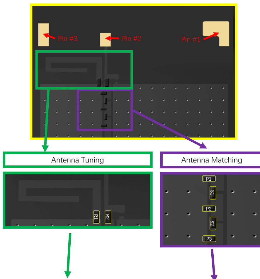
Demo Board Top View
