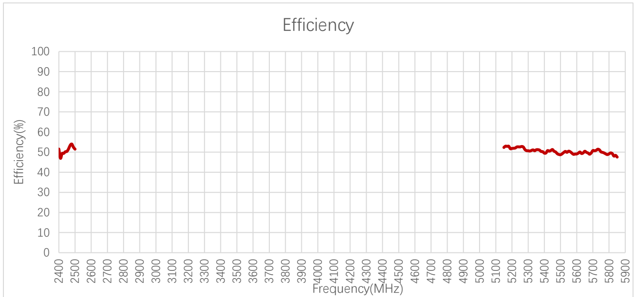
Efficiency (%) - Wi-Fi
