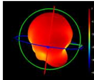
Phi=90 freq=1575MHz
