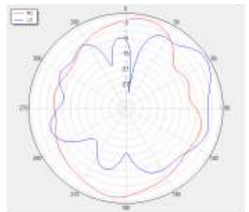
Theta=90 freq=1575MHz
