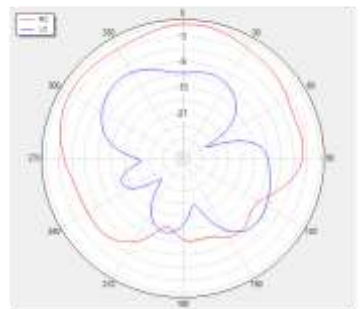
Phi=0 freq=1575MHz
