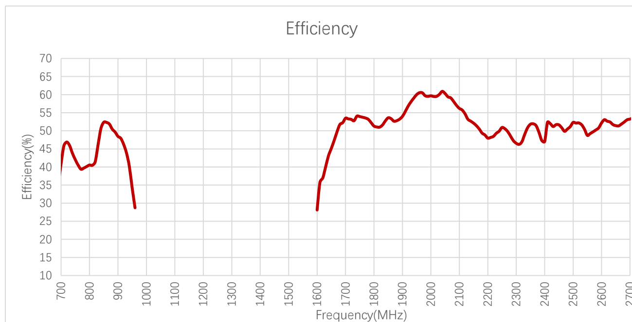
Efficiency (%) - 4G
