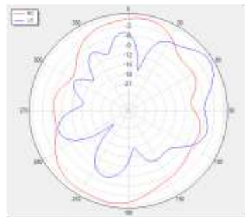
Theta=90 freq=1561MHz
