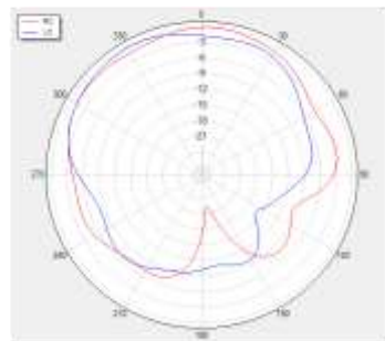
Phi=0 freq=1602MHz
