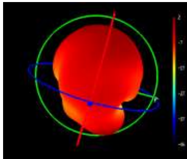
Phi=90 freq=1561MHz
