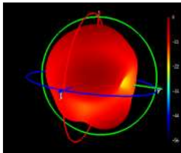
Phi=90 freq=1602MHz
