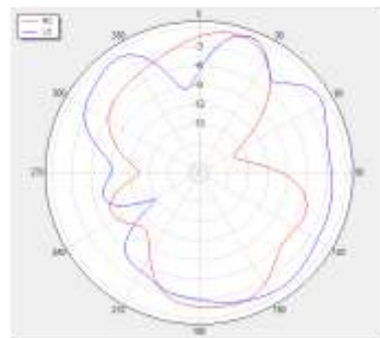
Theta=90 freq=1602MHz
