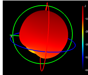
Phi=90 freq=1602MHz
