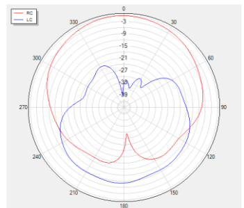
Phi=0 freq=1602MHz
