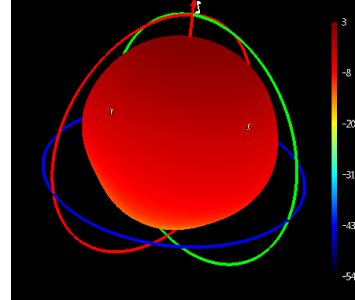
Phi=90 freq=1561MHz
