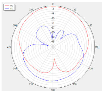
Phi=0 freq=1575MHz
