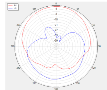
Phi=90 freq=1602MHz
