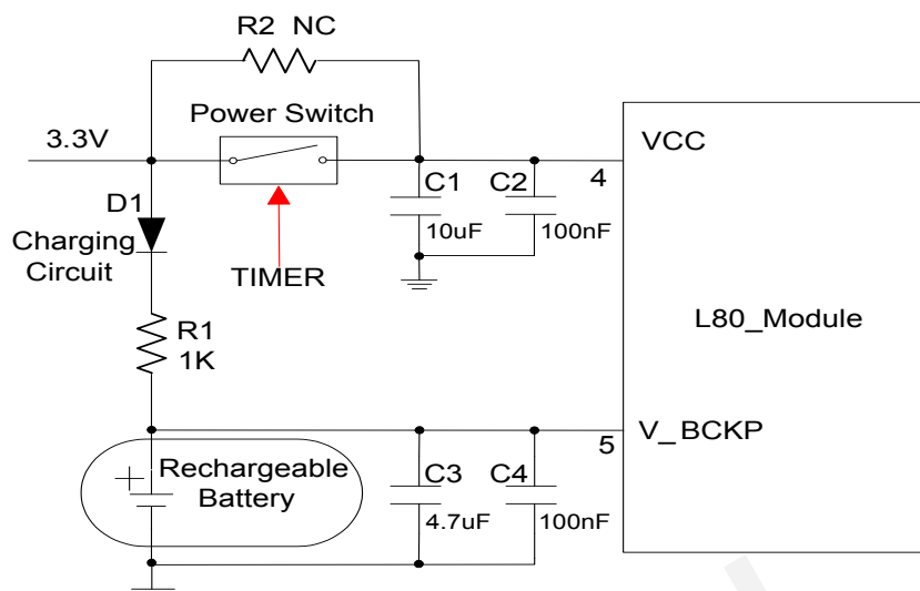
Figure 5: Reference Charging Circuit for Chargeable Battery
