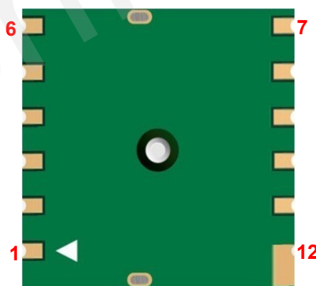
Figure 22: Bottom View of the Module
