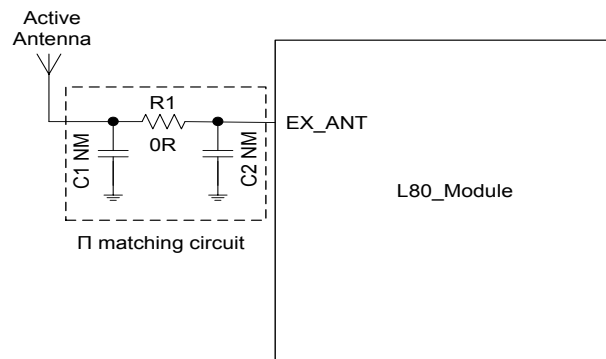
Figure 16: Reference Design for Active Antenna
