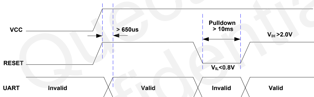
Figure 11: Restart Timing
