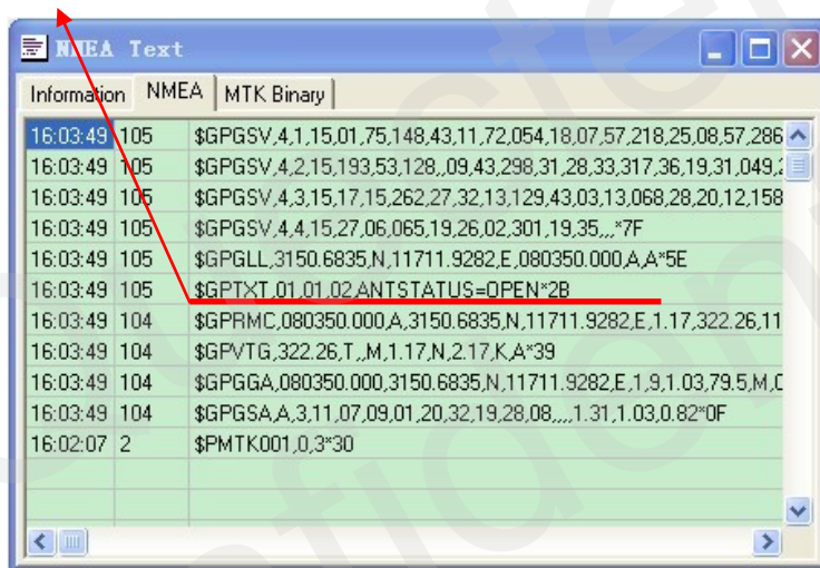
Figure 17: Patch Antenna Status Description in GPSTXT
