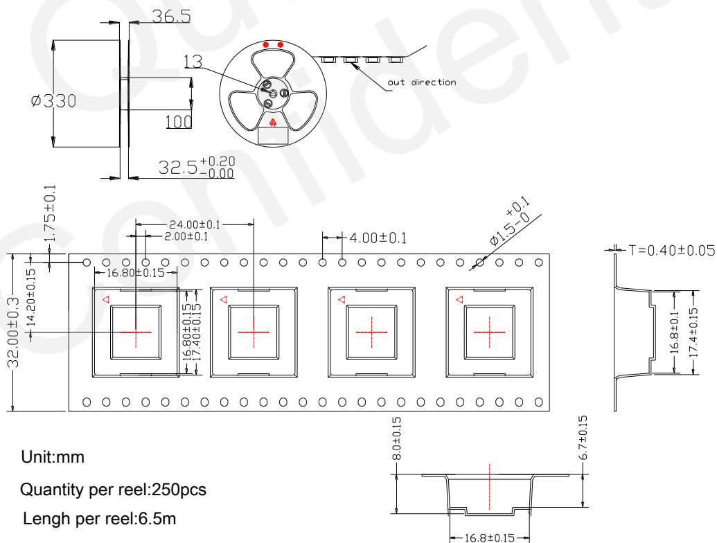
Figure 24: Tape and Reel Specification
