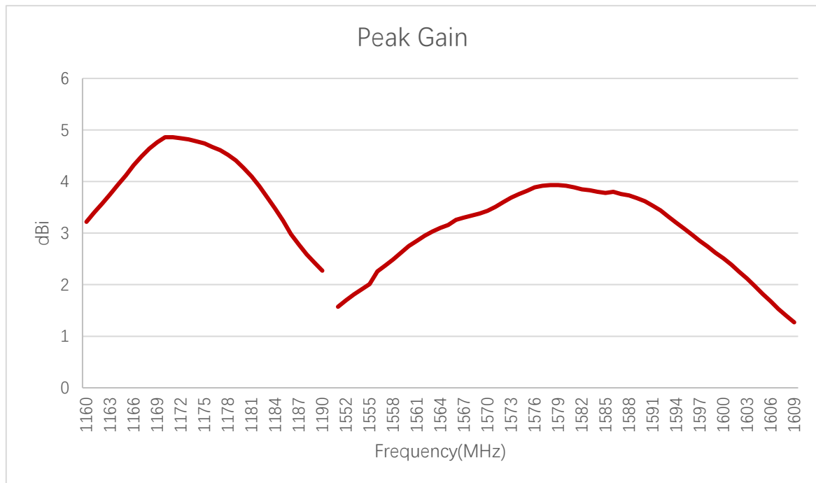
Peak Gain(dBi)-GNSS
