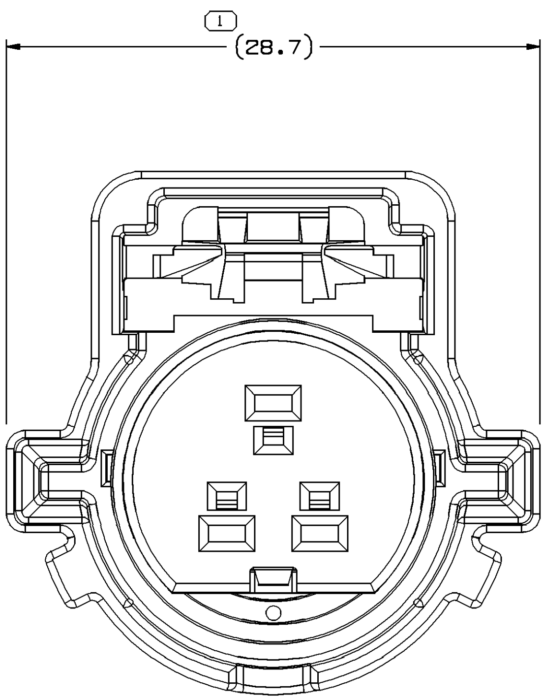
TYPE 102 SAME AS TYPE 101 EXCEPT AS SHOWN
