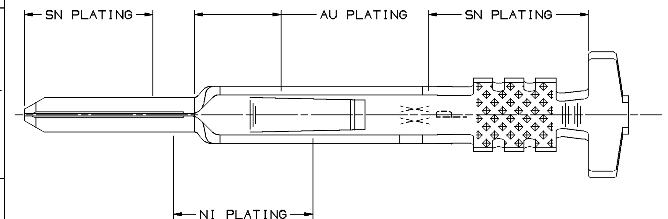
12110502 PLATING LOCATION DETAIL
