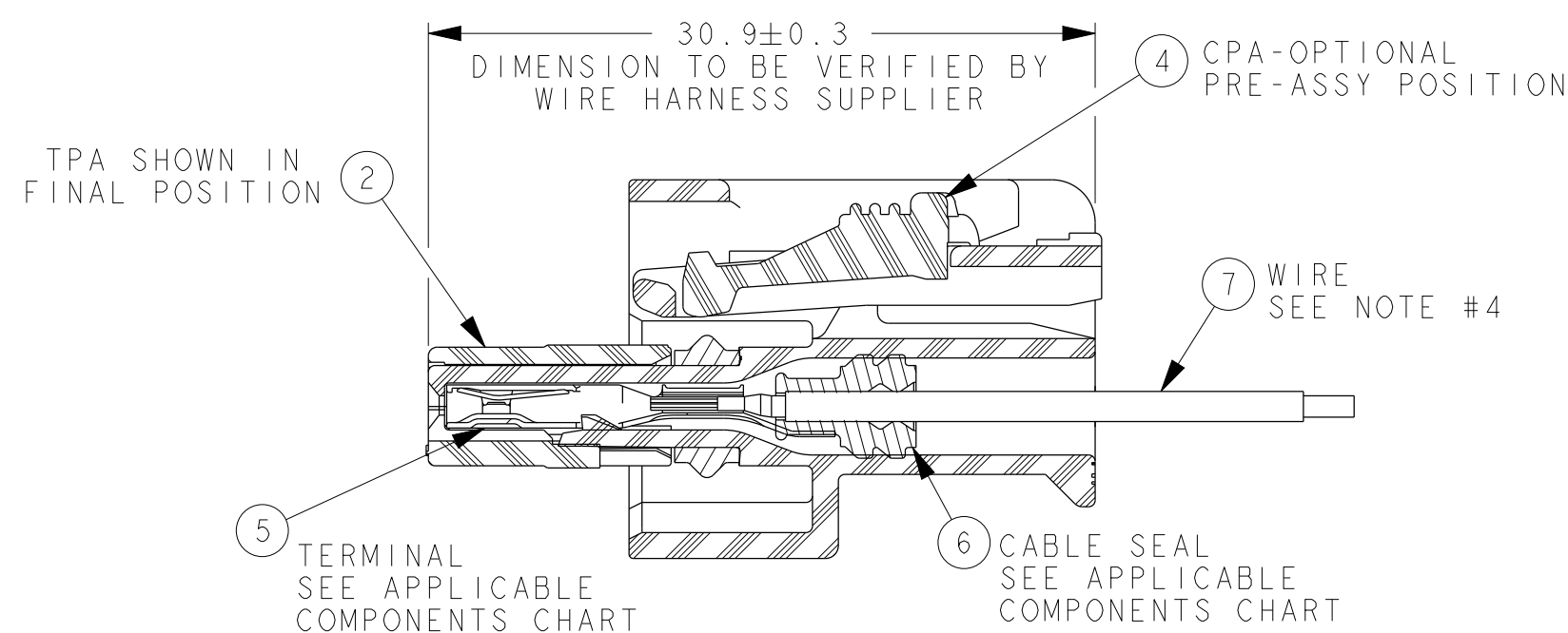
SECTION B-B TPA IN FINAL ASSEMBLY POSITION AS SUPPLIED ON HARNESS
