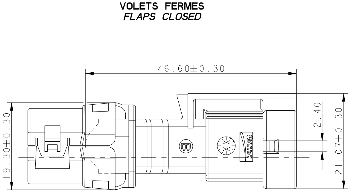
VOLETS OUVERTS POSITION DE LIVRAISON FLAPS OPENED DELIVERY POSITION
