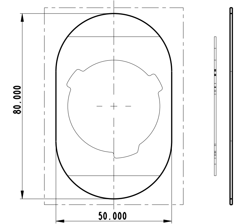
Detail: Free area on the back of Male Holder
