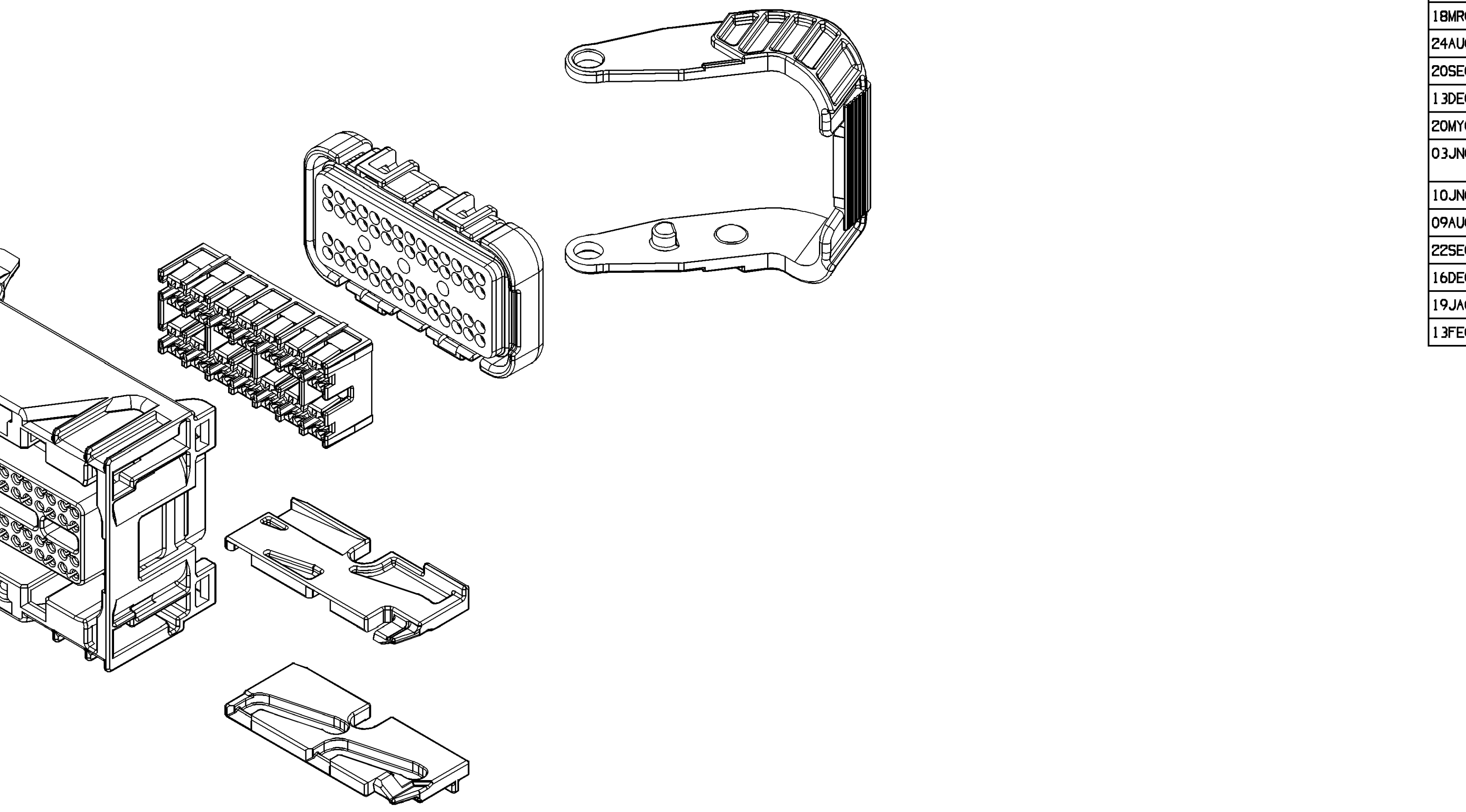
SEMBLY VIEW
