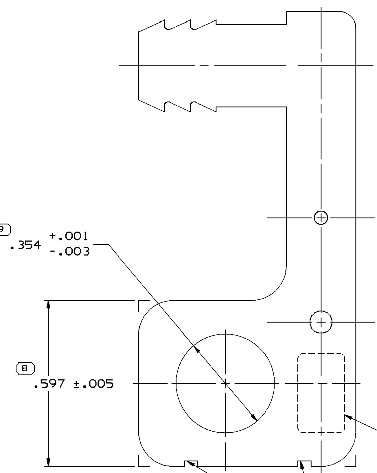
TYPE 407 SAME AS TYPE 401 EXCEPT AS SHOWN
