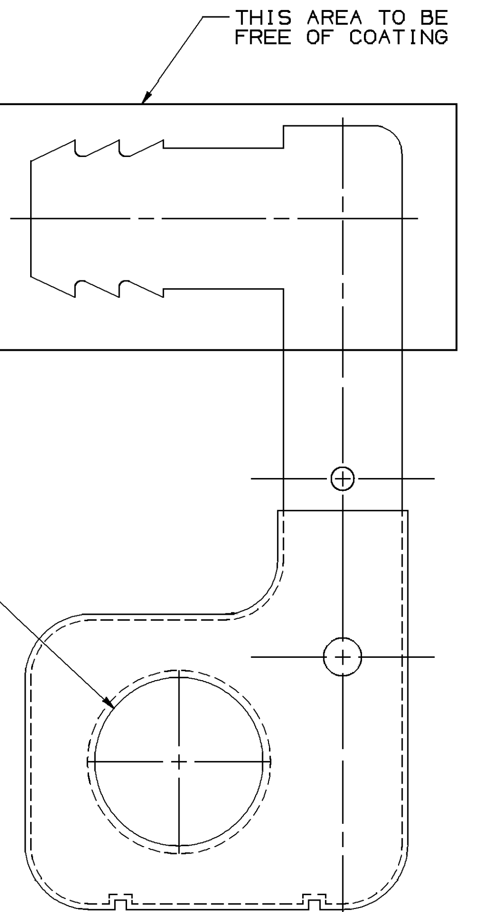
TYPE 409 SAME AS TYPE 407 EXCEPT AS SHOWN
