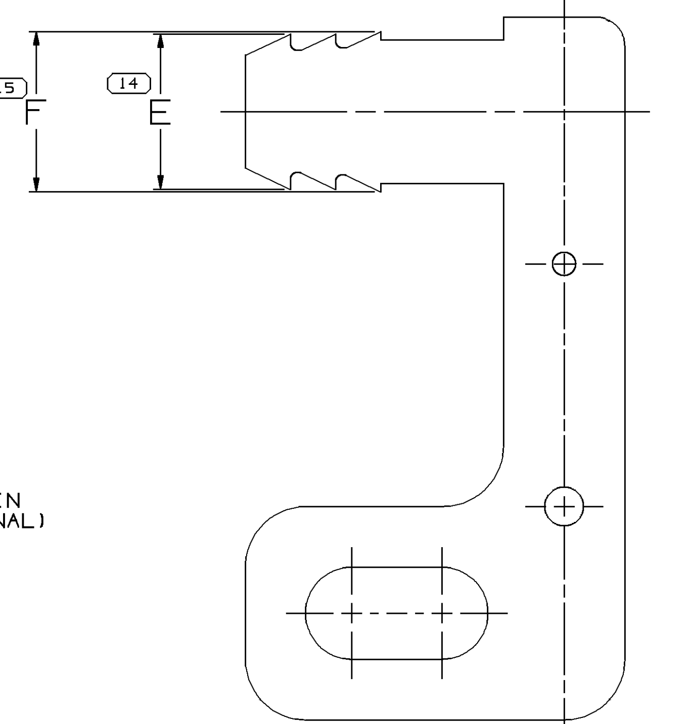
TYPE 408 SAME AS TYPE 401 EXCEPT AS SHOWN
