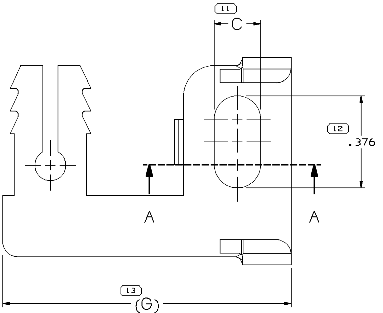
TYPE 402 SAME AS TYPE 401 EXCEPT AS SHOWN
